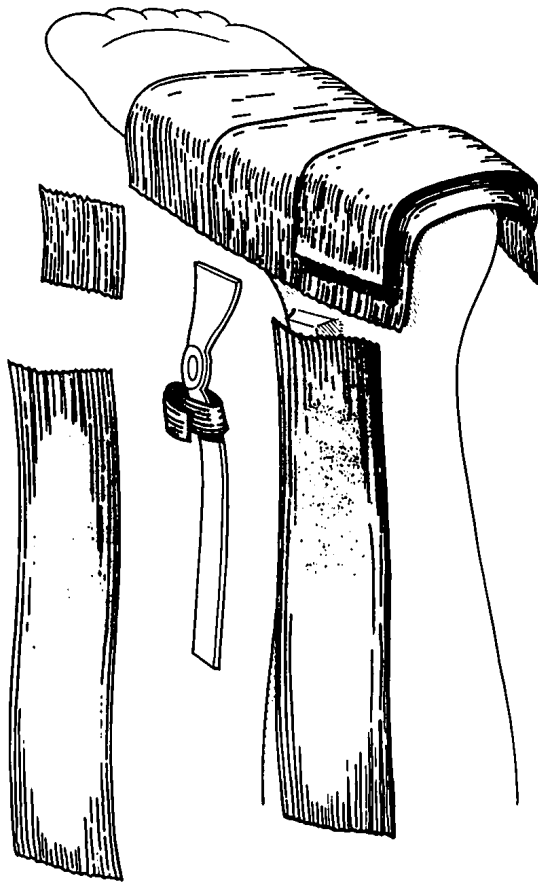
Figure 5. Exploded view of carbon tape and joint lay-up on a modified cast prior to trim.
