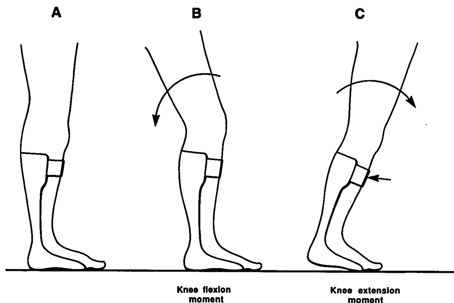
Figure 8. A. A Floor Reaction Orthosis (FRO) in quiet standing; B. A FRO has no effect in maintaining knee stability when the ground force vector passes behind the knee; and C. A FRO imposes knee extension when the ground force vector passes anterior to the knee.
