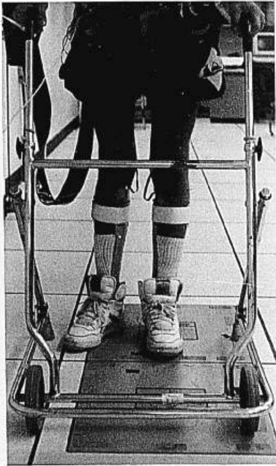
Figure 7. An anterior view of a subject standing using system 1 hybrid orthosis.
