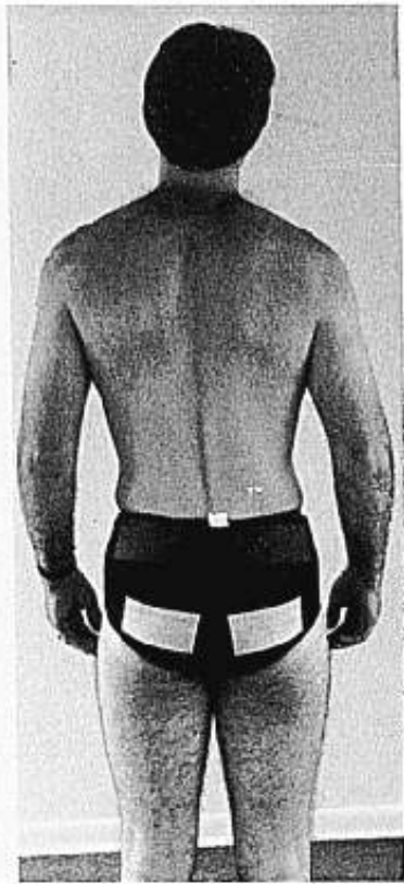
Figure 10. System 3: A pair of briefs incorporates electrodes for bilateral stimulation of the gluteus maximus.
